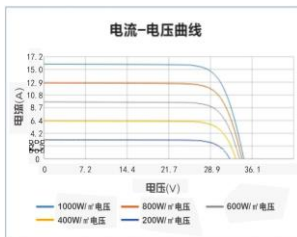
Current-Curves曲线图
