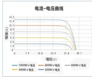
Current-Curves曲线图
