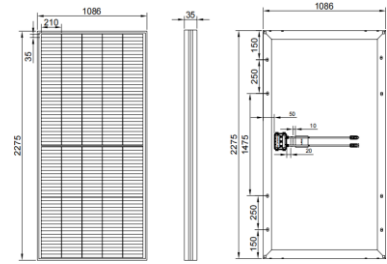
Engineering Drawings 装配图
